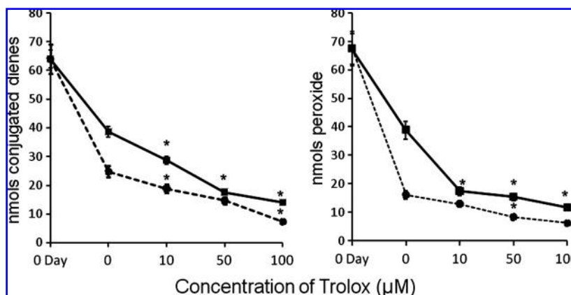
FIG. 3. Effect of Trolox on the decomposition of HPODE. Linoleic acid was oxidized with soybean lipoxygenase, as described in Methods, and was incubated at 37^\circ\text{C} for \leq 72 \text{ h} . Trolox was added as sodium salt at 10\text{-}, 50\text{-}, and 100\text{-}\mu\text{M} levels. At specified time periods, lipid peroxides and conjugated dienes were determined. The left and the right panels represent conjugated dienes and peroxides, respectively. Squares and circles, values at 1- and 2-day incubations. The data are expressed as average \pm SD from six different sets of incubations. *Values significantly different from control (0 time) values.
