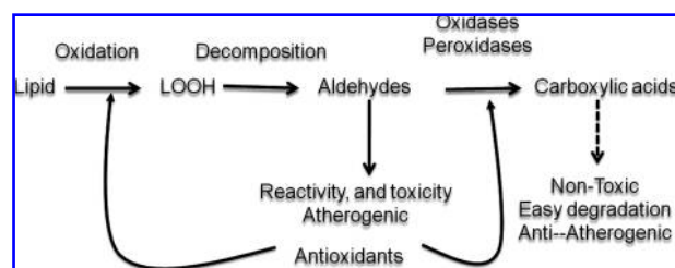
FIG. 8. Antioxidants might prevent the oxidation of aldehydes into carboxylic acids.
