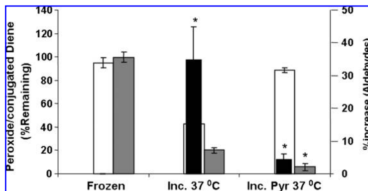
FIG. 2. Decomposition of HPODE in serum. HPODE was prepared ( \sim 30 \mu\text{mol} ); an aliquot was set aside for peroxide, conjugated diene, and aldehyde determinations. Dried HPODE was re-suspended in fetal calf serum at a concentration of 1.0 \mu\text{mol} in 100 \mu\text{l} and aliquoted into 96-well microtiter plates. Aliquots were also stored at -20^\circ\text{C} . When needed, pyruvate was added in 5\text{-}\mu\text{l} quantities to give a final concentration of 5.0 \mu\text{mol} per 100 \mu\text{l} . Samples were collected at 1, 2, and 3 days after incubation at 37^\circ\text{C} for analytic determinations. Incubations were set in quintuplicates, and the values represent average \pm SD. *p < 0.05 versus sample incubated at 37^\circ\text{C} . Open bars, grey bars, and black solid bars represent conjugated dienes, peroxides, and aldehydes, respectively.
