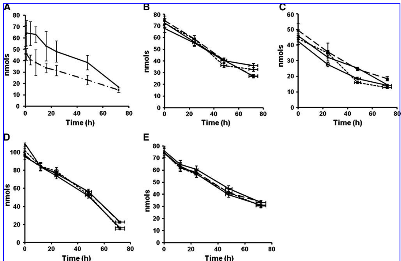
FIG. 1. The decomposition of 13-HPODE with time. Linoleic acid was oxidized with soybean lipoxygenase, as described in Methods, and was incubated at 37°C for <72 h. At specified time periods, lipid peroxides and conjugated dienes were determined. (A) The determination of peroxides (■) and conjugated diene (◆) during the decomposition of HPODE. The data are expressed as average \pm SD from six different sets of incubations. (B, C) Determination of peroxides and conjugated dienes in the presence of \alpha -tocopherol at 0 (◆), 5 (■), 25 (▲), and 100 (×) \mu\text{M} concentrations. (D, E) Determination of peroxides and conjugated dienes in the presence of BHT at 0 (◆), 10 (■), 50 (▲) and 100 (×) \mu\text{M} concentrations. The (B–E) values are too close, and the results are averages from four independent trials.
